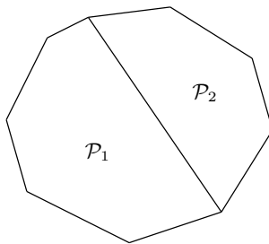
Fig. 2.6. Decomposition of a polygon into two.
