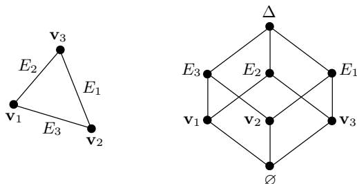
Fig. 5.1. The face lattice of a triangle.
