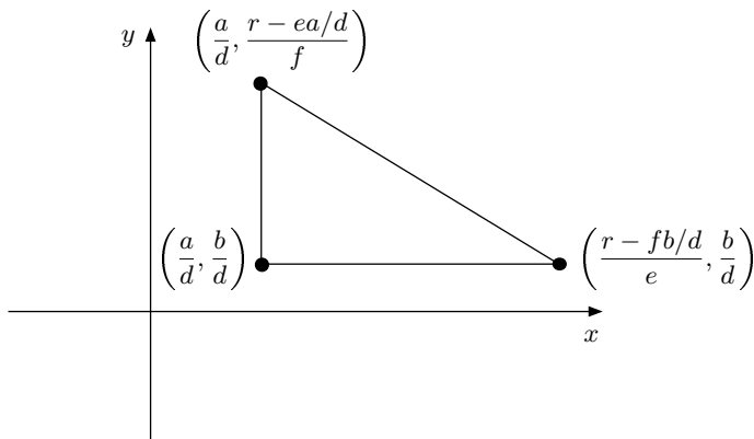
Fig. 2.9. A right rational triangle.
